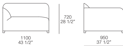
terminale sx-dx/left-right end-units
